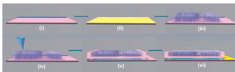
Figure 1. Fabrication flowcharts of a GaN NW LED device, including (i) growth of a p-type GaN thin film on (0001) sapphire, (ii) Au catalyst thin-film evaporation, (iii) growth of n-type GaN NWs, (iv) piezoelectric investigation with an atomic force microscope, (v) spin-coating of a polymer spacer (PMMA) in the LED device, and (vi) deposition of InO and Au/Ni electrodes for n-type and p-type contact, respectively.
